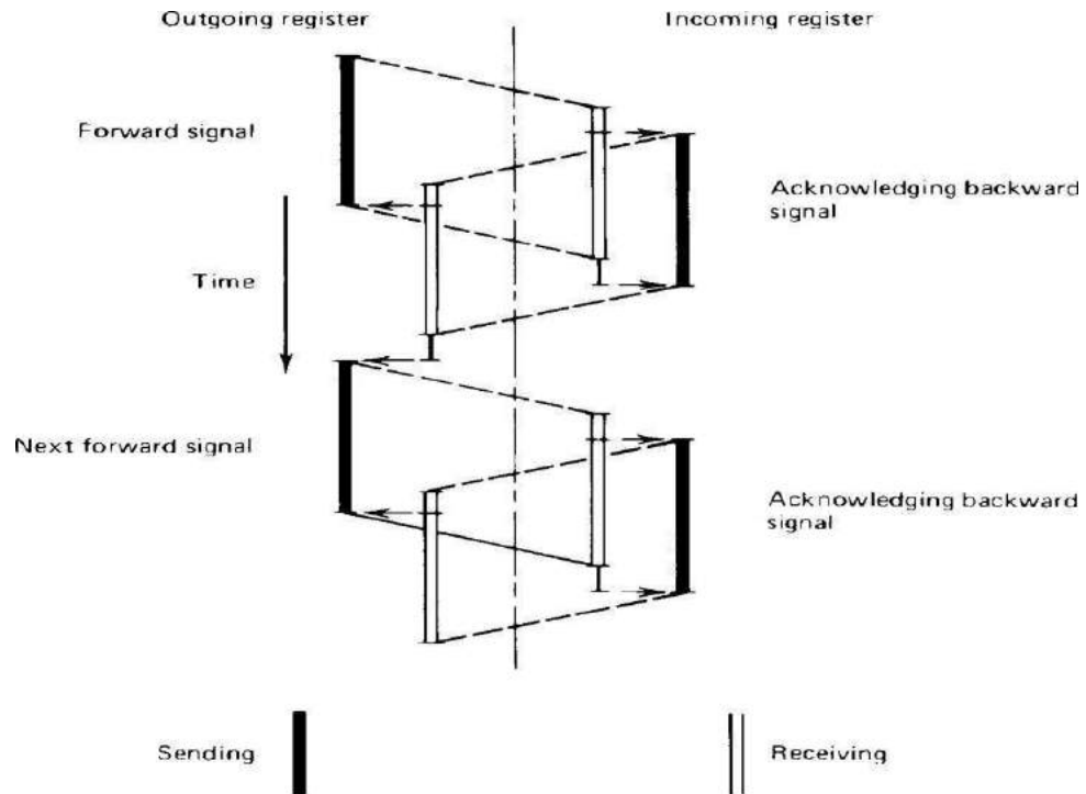
Figure 2.4 Fully compelled signaling procedure.
