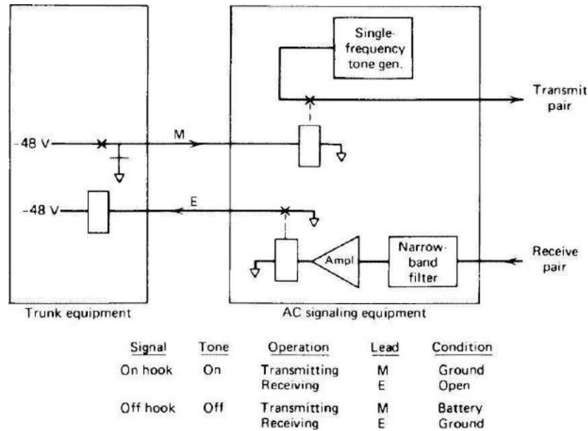
Fig: 2.1 Functional block diagram of an SF signaling circuit. Note: Wire pairs “receive” and “transmit” derive from the FDM multiplex equipment. Note also the E-lead and M-lead.
