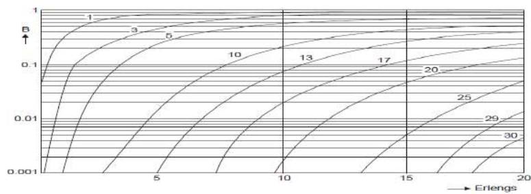
Plot of B(N, A) .
