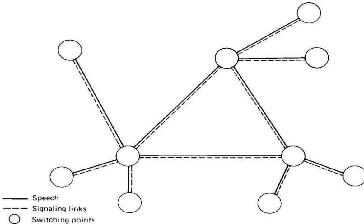
Figure 2.6 Quasi-associated channel signaling, typical of E-1 channel 16.
