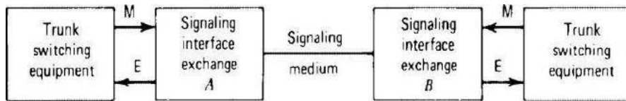
Figure 2.3 E&M signaling.
