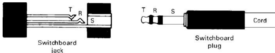
Figure 2.10 Switchboard plug with corresponding jack (R, S, and T are ring, sleeve, and tip, respectively).
