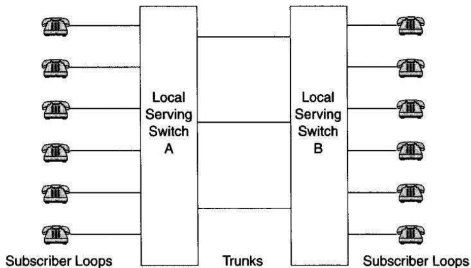
Fig: 1.6. Subscriber loops connect telephone subscribers to their local serving exchange trunks interconnect exchanges (switches).
