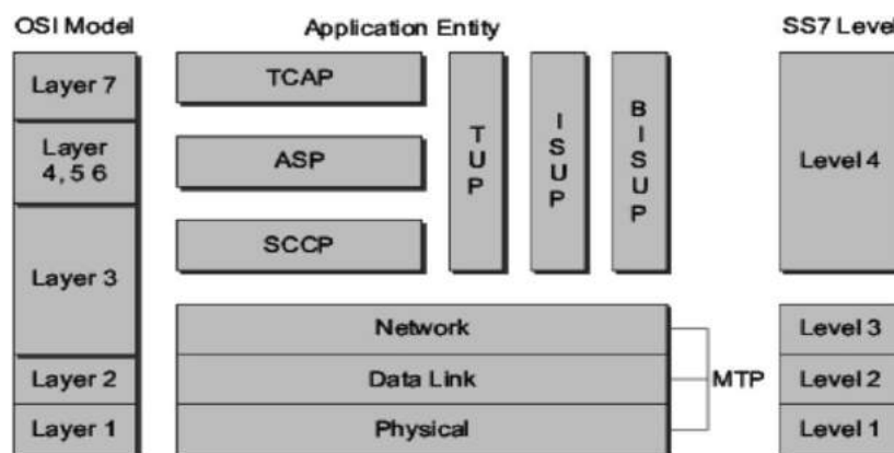
Fig:2.11 SS7 Layers
