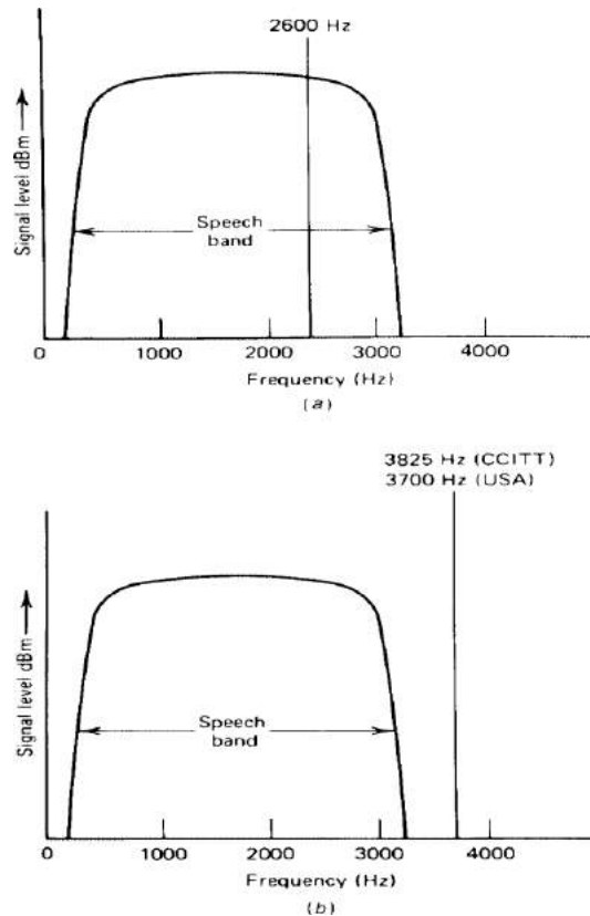
Fig: 2.2 SF signaling (a) in-band and (b) out-of-band.
