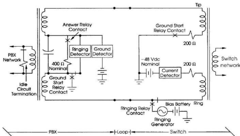
Figure 2.9 Ground-start interface block diagram.
