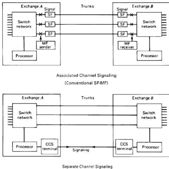
Figure 2.8 Conventional analog associated channel signaling ( upper ) versus separate channel signaling (which we call quasi-associated channel signaling)
