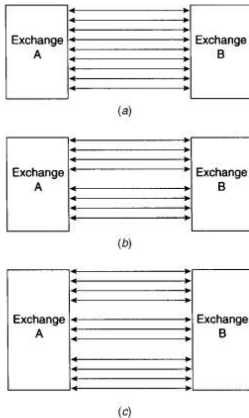
Fig: 1.10 Two-way and one-way circuits: two-way operation (a), one-way operation (b), and a hybrid scheme, a combination of one-way and two-way operation (c).
